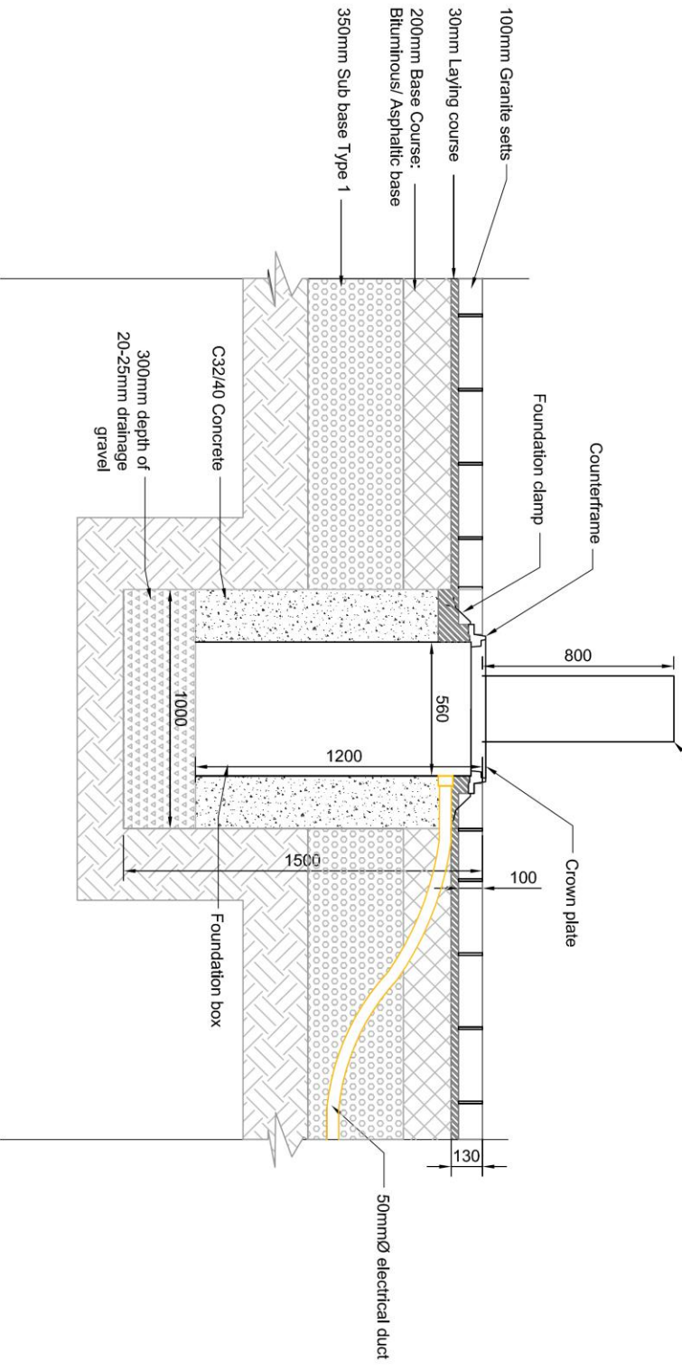
CROSS SECTION
